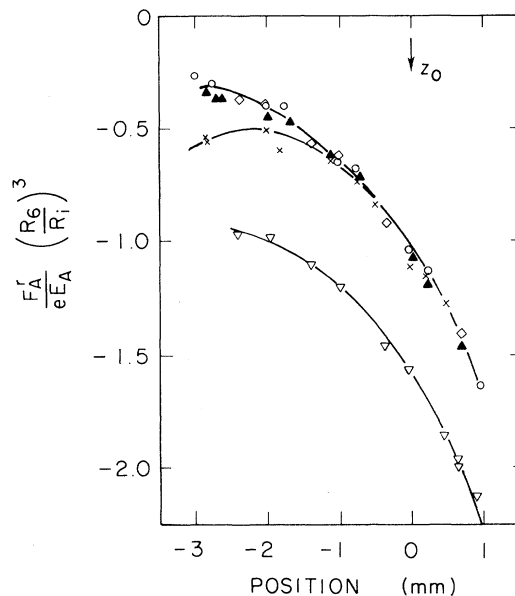
FIG. 2. (F_A^r / eE_A)(R_6/R_i)^3 vs position for the five balls in set 1 of cooldown 2. R_i = radius of ball i . Symbols: ball 10 (circles); ball 6 (crosses); ball 11 (solid triangles); ball 12 (diamonds); ball 13 (open triangles). The departure of the crosses from the upper curve is due to P_z \sim 5 \times 10^{-8} esu cm on ball 6. The effect of P_z is zero at z_0 where \partial E_A/\partial z = 0 . \frac{1}{3}e for ball 13 corresponds to 0.58 on the vertical axis.
